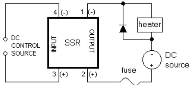
Figure 2 Wiring Diagram
