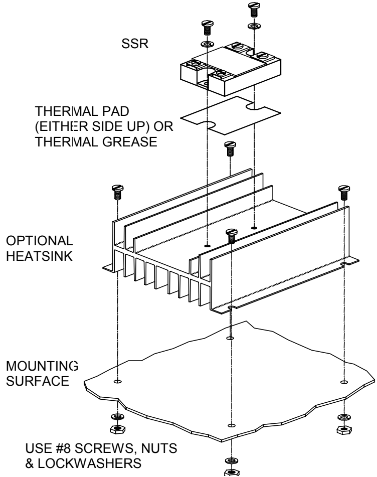
Figure 1 Assembly of an SSR to an optional heatsink
